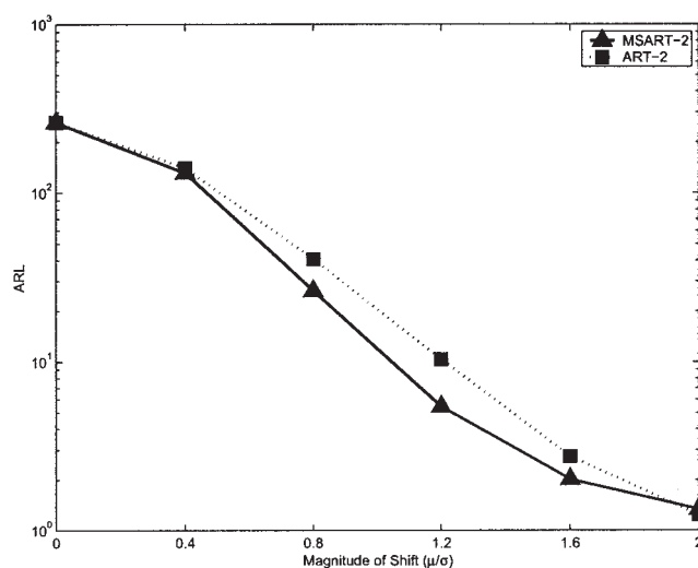
Figure 8. Comparison of ART-2 and MSART-2 performances based on ARL for a linear multivariate process.
