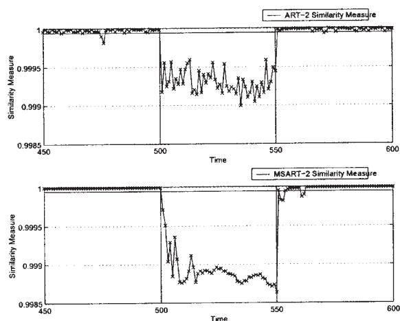
(c) ART-2 and MSART-2 Measures of Similarity
