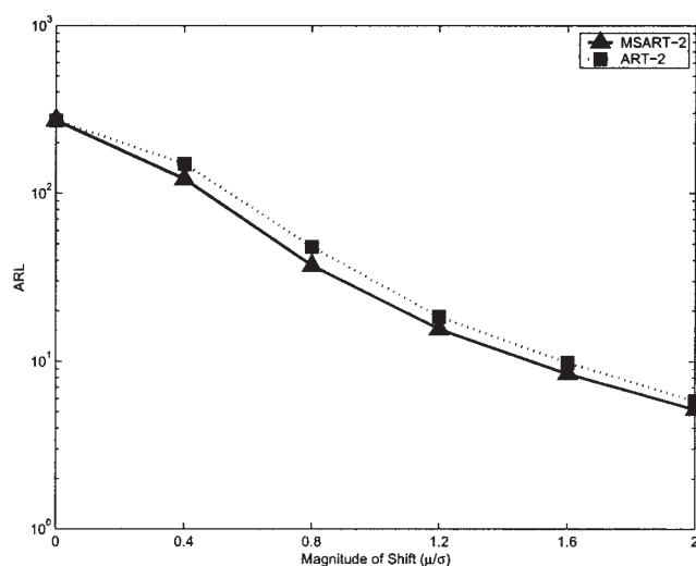
Figure 9. Comparison of ART-2 and MSART-2 performances based on ARL for a nonlinear multivariate process.
